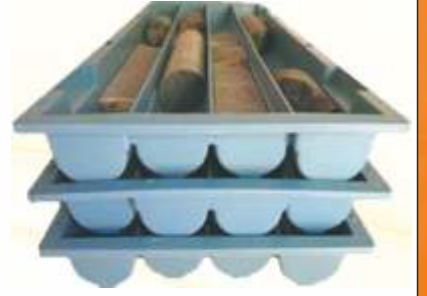
Without lids, just rotate trays. They do not touch core below.
